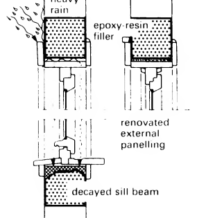
⑪ Moisture damage to outer cladding
